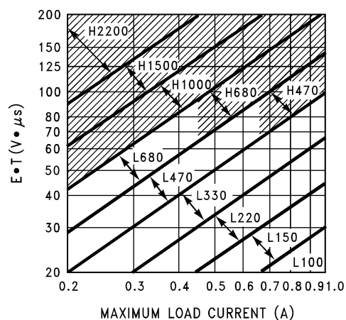
Figure 31. LM2575(HV)-ADJ
